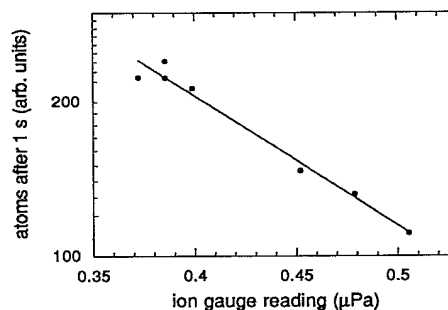
FIG. 5. Number of atoms that survive 1 s of trapping at 50 W microwave power, as a function of the ion gauge reading inside the vacuum chamber. The straight line represents exponential decay.
