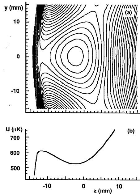
FIG. 2. (a) Calculation of the trapping potential in a vertical plane containing the symmetry axis of the microwave mode ( Oyz plane; z is vertical). For this calculation the microwave power is 50 W. Contour lines are drawn 20 \mu\text{K} apart. (b) Cut of the same potential along the z axis ( y=0 ).
