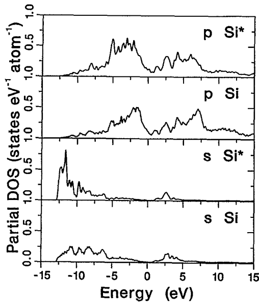
FIG. 2. Local, Si site projected, partial densities of states for \text{TiSi}_2 , as calculated for the ground state and for the excited state with the presence of a core hole. The latter are indicated by an asterisk.
