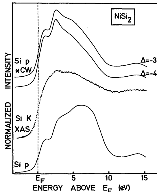
FIG. 10. Comparison of the experimental Si K XAS spectrum of \text{NiSi}_2 (dots) with the partial density of Si p states, and the partial density of unoccupied Si p states treated by the Clogston-Wolff model with \Delta set at -3 and -4 eV.
