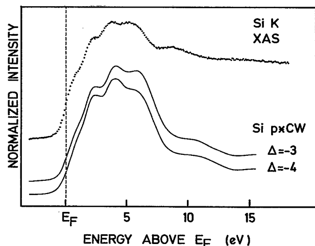
FIG. 8. Comparison of Si K XAS curves and simulations based on the density of unoccupied Si p states and the generalized CW model with \Delta = -3 and -4 eV for \text{TiSi}_2 .
