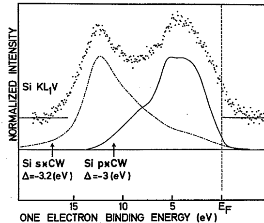
FIG. 7. Simulations of the local density of Si s and p states at a core ionized site using the ground-state DOS of \text{TiSi}_2 and an attractive core-hole potential in the generalized Clogston-Wolff model. The CW curves are compared with the experimental KL_1V Auger spectrum. The theoretical curve broadening is as for the AES curve in Fig. 3.
