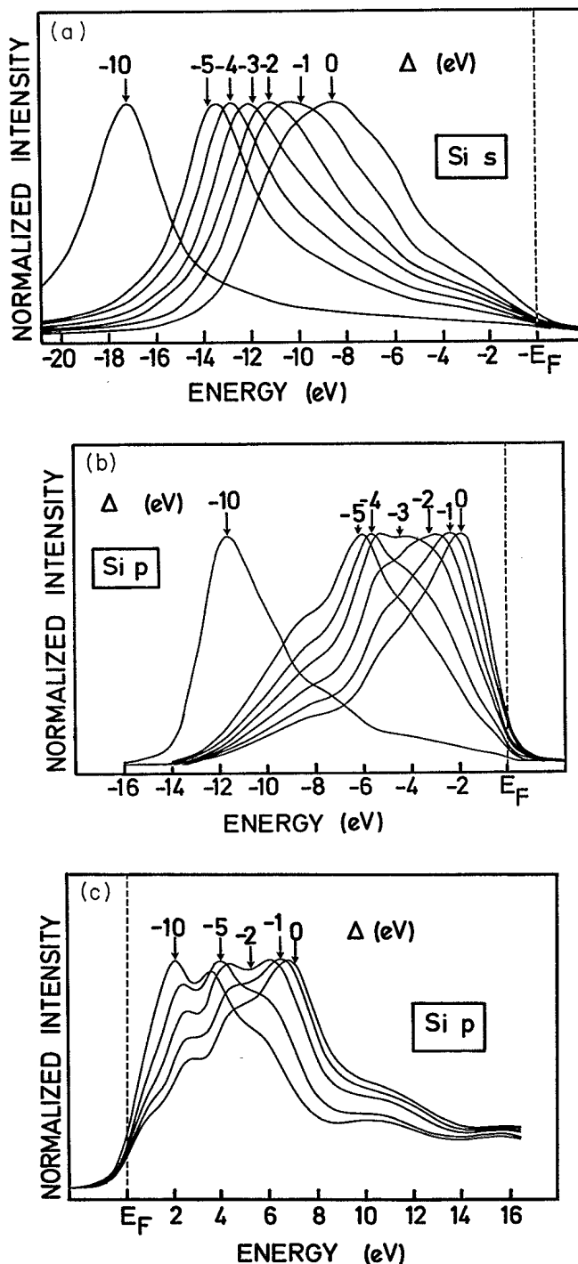
FIG. 6. Clogston-Wolf simulations of the distortion of the local partial density of Si states at a core ionized site using the ground-state DOS of \text{TiSi}_2 . (a) Occupied s states; (b) occupied p states, and (c) unoccupied p states. The theoretical curve broadening is as described in Sec. II B.
