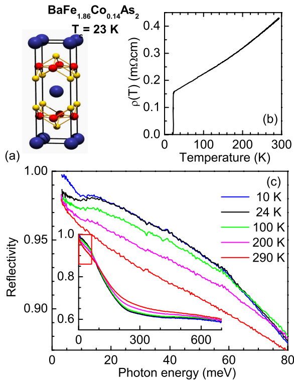
Fig. 1: (Colour on-line) (a) Unit cell of the tetragonal BaFe 2 As 2 structure. Magnetic susceptibility measured with H = 10 Oe. (b) Temperature dependence of the resistivity. (c) Far-infrared reflectance for selected temperatures. Note the strong increase in reflectance below 10 meV for data taken at 10 K in the SC state.
