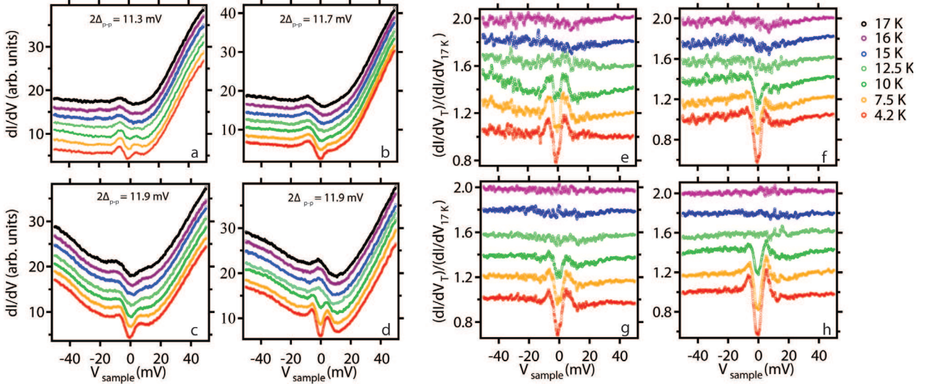
Fig. 3: (Colour on-line) Overdoped \text{BaCo}_x\text{Fe}_{2-x}\text{As}_2 ( x=0.21 , T_c=13\pm 1 K): (a)–(d) STS spectra taken at four different positions. All spectra taken above T_c fall perfectly on top of each other, contrary to those taken below T_c . (e)–(h) The spectra shown in (a)–(d) normalised to the respective spectra taken at 17 K, i.e. > T_c .
