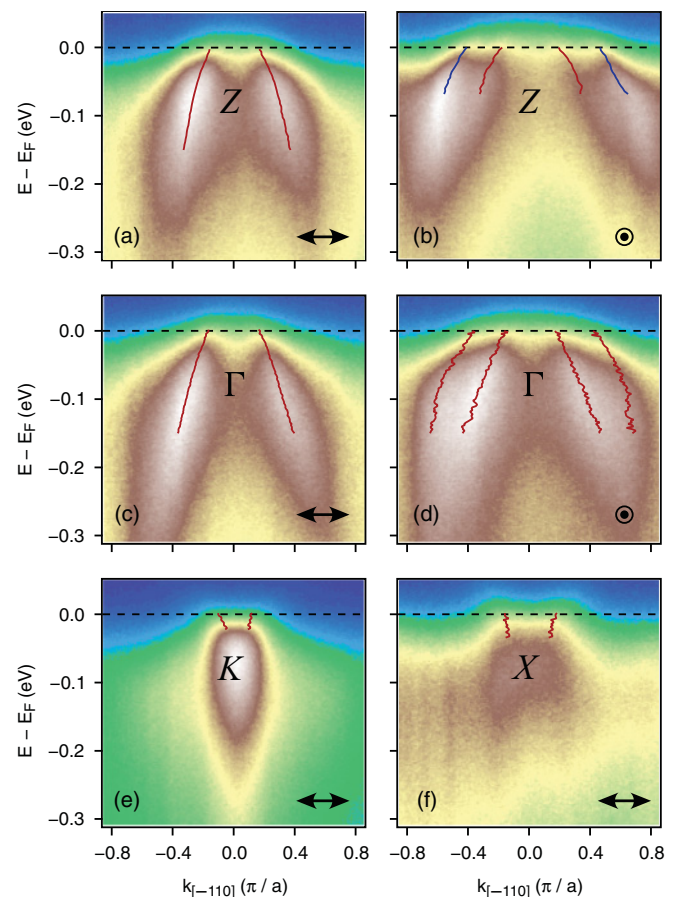
FIG. 4. (Color online) ARPES energy distribution maps near the high-symmetry points \Gamma, X, Z , and K of the parent compound \text{EuFe}_2\text{As}_2 taken in the paramagnetic state at T = 220 K. The data near Z and \Gamma were recorded using both s - and p -polarized photons. The data near K and X were obtained using s -polarized photons.
