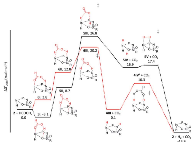
Fig. 8 Potential energy diagram (DFT, BP86, def2-TZVP) for dehydrogenation of formic acid by 5I (black profile) and 6I (red profile); \Delta G_{298K}^\circ is in kcal mol −1 .
