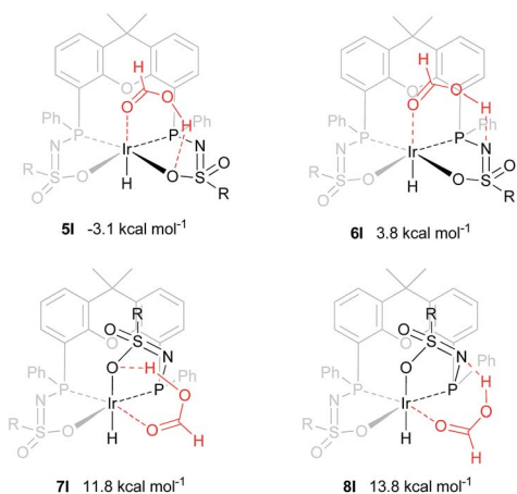
Fig. 7 DFT optimized geometries of formic acid adducts 5I – 8I (BP86, def2-TZVP, \Delta G_{298K}^\circ in kcal mol −1 ), R = phenyl.
