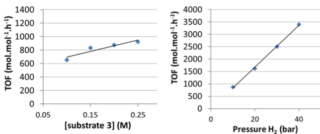
Figure 9. Left: TOF (in \text{mol mol}^{-1} \text{h}^{-1} , calculated at 15% conversion) as a function of the substrate S3 concentration. Right: TOF (in \text{mol mol}^{-1} \text{h}^{-1} , calculated at 15% conversion) as a function of the dihydrogen pressure observed for substrate S3 .
