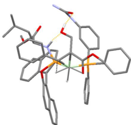
Figure 13. Optimized structure of the hydride migration transition state TS3 ( \Delta G_{298\text{K}} = +20.9 \text{ kcal mol}^{-1}/2 , \nu^\ddagger = 626.2i \text{ cm}^{-1} ). Hydrogen bonds are drawn in orange. The black dotted line represents the hydride insertion to form the alkyl hydride species 6.
