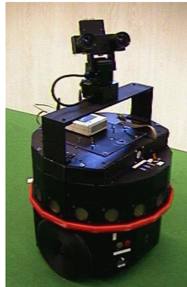
Figure 6: Our robot with the stereo head used to take images and disparity maps.
