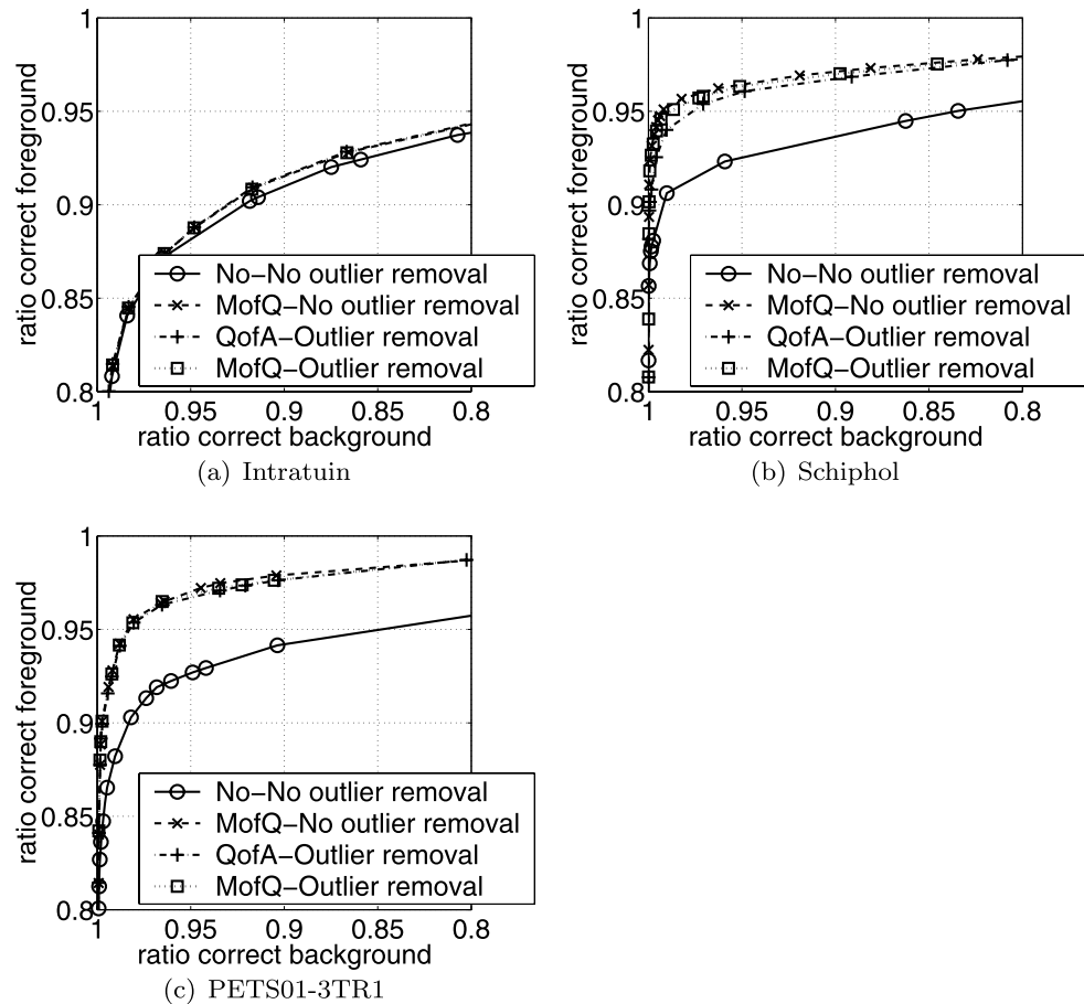
Fig. 6 Total-ROCs of the classification results on real data with different values of update speed and threshold. Only a selection of the methods is shown as most methods coincide
