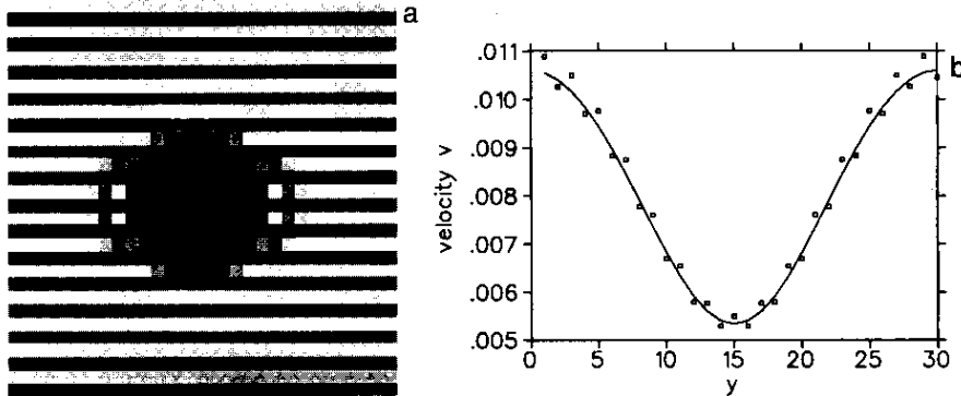
FIG. 9. The results for fluid flow around a sphere. The velocity field in a plane which bisects the sphere is analyzed. Fluid is flowing from left to right, and periodic boundaries are used in both directions. (a) The relative difference \Delta v between the velocity fields obtained by the D_3Q_{19} and D_3Q_{15} models. The colours run from gray to white with the scale -3.0\% \leq \Delta v \leq 3.0\% . (b) The velocity profile at the inlet for both models. The solid line and open boxes show the results for the D_3Q_{19} and D_3Q_{15} models, respectively.
