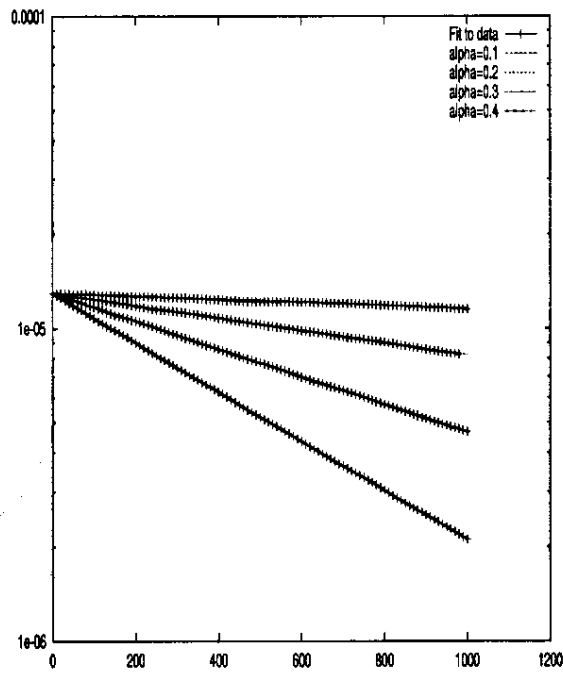
Fig. 3. The decay of the velocity in time at coordinate (\frac{L}{4}, \frac{W}{2}) for different values of \alpha .
