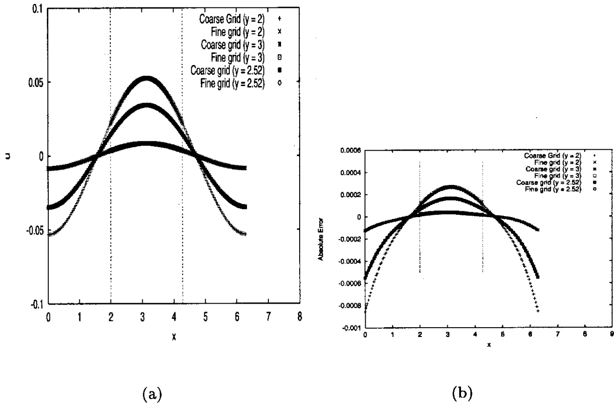
Fig. 6. The velocity at three lines parallel to the x -axis on both grid resolutions and the corresponding absolute errors at t = 2000 . The region between the dashed lines contains the fine grid.
