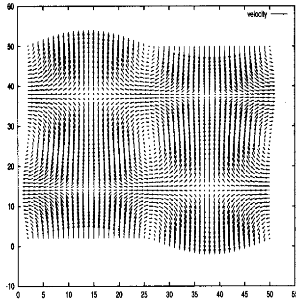
Fig. 2. The initial velocity u_x in the Taylor vortex benchmark.
