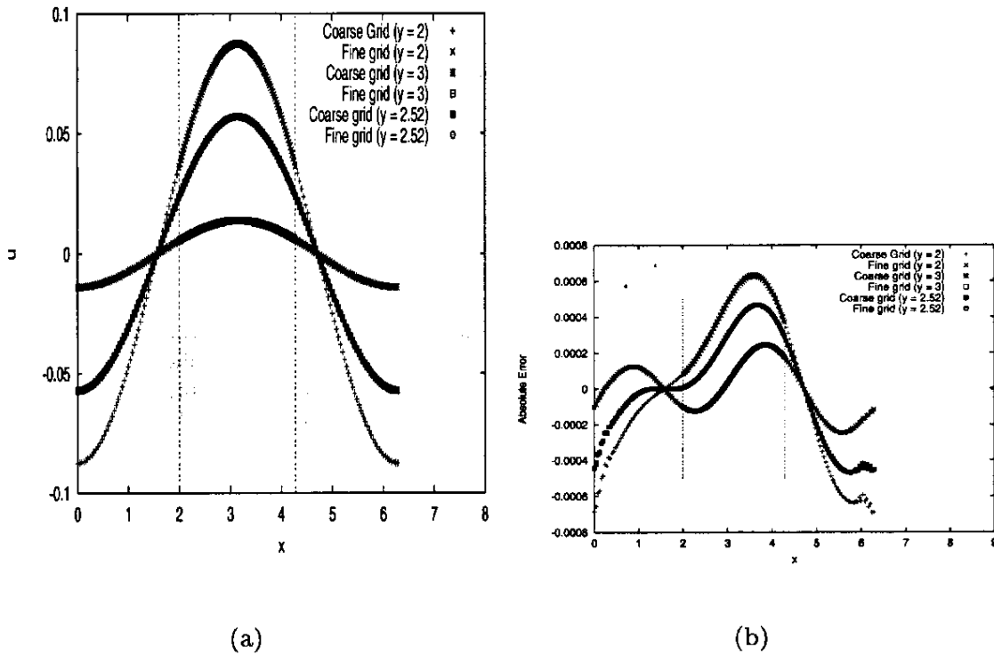
Fig. 4. The velocity at three lines parallel to the x -axis on both grid resolutions and the corresponding absolute errors at t = 100 . The region between the dashed lines contains the fine grid.
