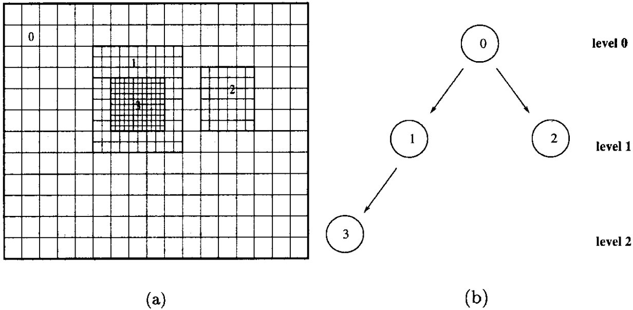
Fig. 1. On the left an example of a nested grid is shown and on the right the corresponding hierarchical structure is depicted.
