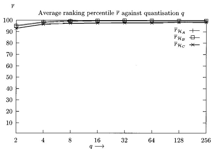
Fig. 5. Average ranking percentile of c_4c_5c_6 denoted by \bar{r}_{\mathcal{H}_A} , l_4l_5l_6 given by \bar{r}_{\mathcal{H}_B} and color invariant edge maxima denoted by \bar{r}_{\mathcal{H}_C} , plotted against quantization q .
