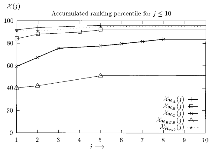
Fig. 7. Accumulated ranking \mathcal{X} plotted against ranking j with q = 16 for c_4c_5c_6 denoted by \mathcal{X}_{\mathcal{H}_A} , l_4l_5l_6 denoted by \mathcal{X}_{\mathcal{H}_B} , color edges given by \mathcal{X}_{\mathcal{H}_C} , RGB given by \mathcal{X}_{\mathcal{H}_{RGB}} , and normalized color rgb denoted by \mathcal{X}_{\mathcal{H}_{rgb}} .
