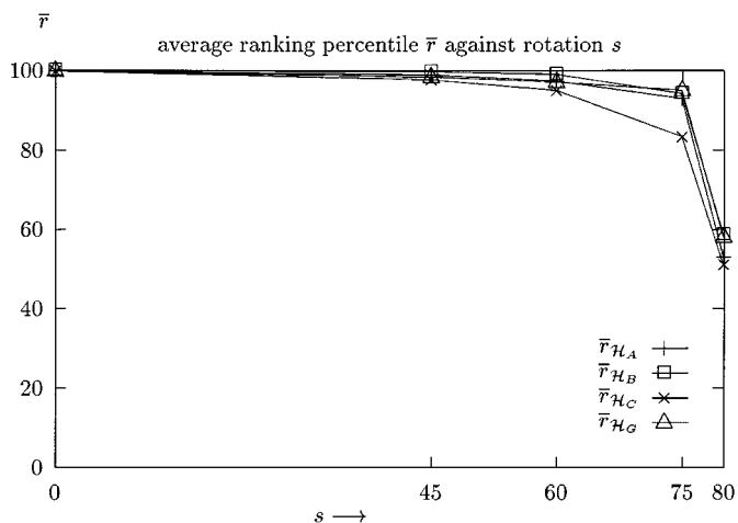
Fig. 12. Ranking percentile plotted against the angle of rotation s denoted by \bar{r}_{\mathcal{H}_A} , \bar{r}_{\mathcal{H}_B} , \bar{r}_{\mathcal{H}_C} , and \bar{r}_{\mathcal{H}_G} .
