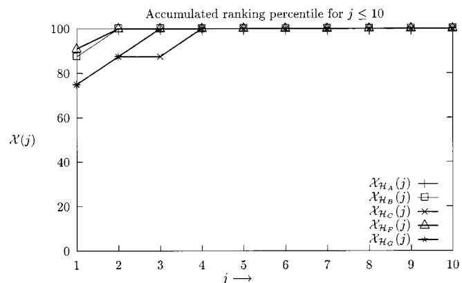
Fig. 13. Discriminative power plotted against the ranking j for \bar{r}_{\mathcal{H}_A} , \bar{r}_{\mathcal{H}_B} , \bar{r}_{\mathcal{H}_C} , \bar{r}_{\mathcal{H}_F} , and \bar{r}_{\mathcal{H}_G} .
