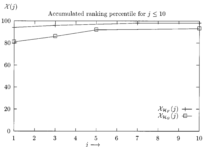
Fig. 8. Accumulated ranking plotted against ranking j with q = 16 for combined color-shape invariants \mathcal{X}_{\mathcal{H}_F} and \mathcal{X}_{\mathcal{H}_G} .
