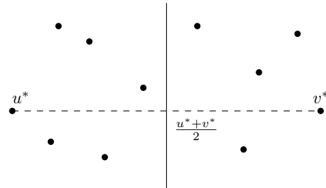
Figure 1. During metric tree construction, the pair of points with maximal distance is selected to guide the splitting of the current node.
