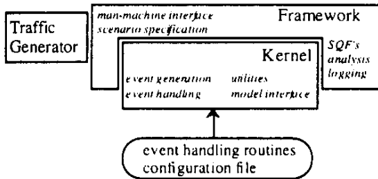
FIGURE 3: ADS-SIM DESIGN
