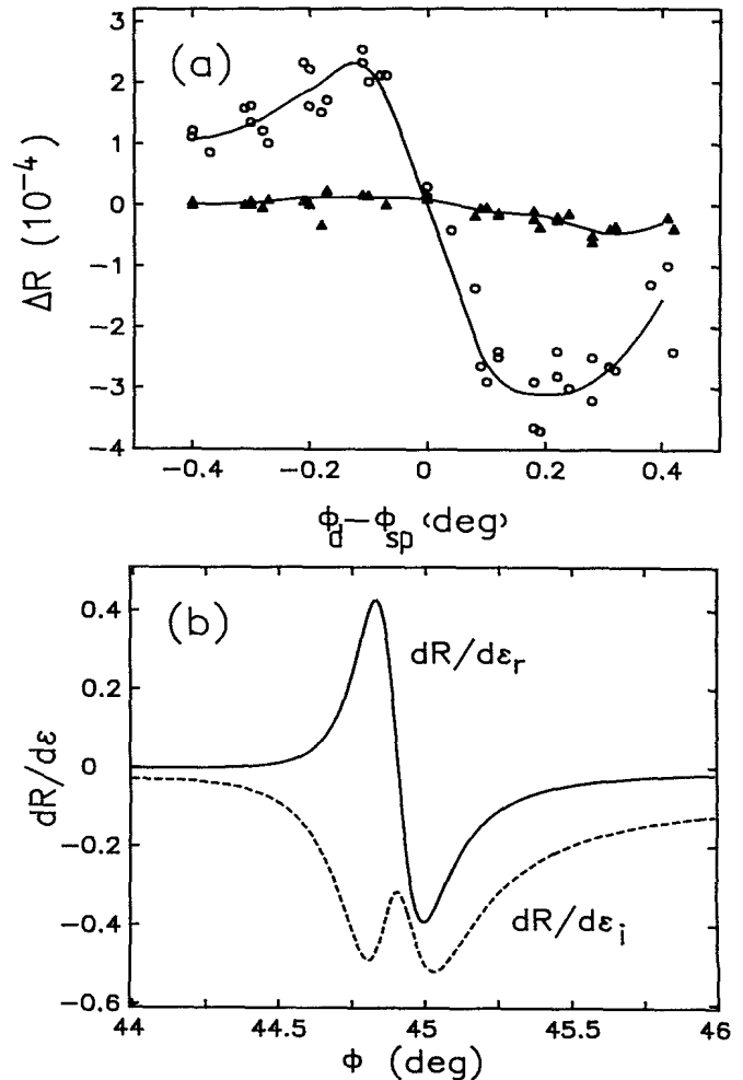
FIG. 3. (a) Measured change of reflectivity \Delta R vs the angle of detection \Phi_d relative to the angle at SP resonance \Phi_{Sp} . The circles mark \Delta R at its maximum around zero delay time (peak level); the triangles mark \Delta R at a delay time \approx 3 ps (plateau level). The lines are a guide to the eye. (b) Calculated derivative of the reflectivity R with respect to the real and imaginary parts of the dielectric constant of the silver of the film, vs the angle of incidence.
