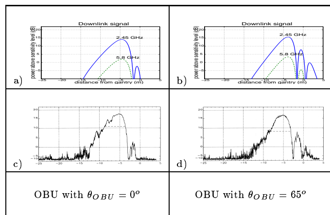
Fig. 6. Calculations and measurements of the received power for two values of OBU orientation \theta_{OBU} . The measurements are taken from [4, page A.13 & A.14].
