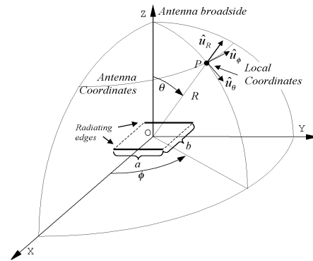
Fig. 5. Geometry for far-field pattern of rectangular microstrip patch.) Philips/Kista system.
