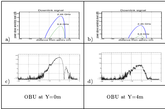
Fig. 3. Calculations and measurements of the received power for two values of Y. The measurements are taken from [4, page A.1 & A.9].
